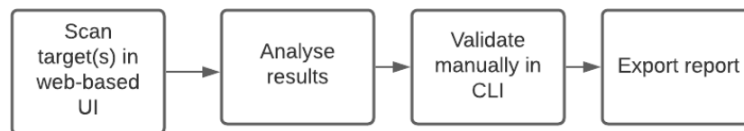
Figure 1: Workflow ([6])
